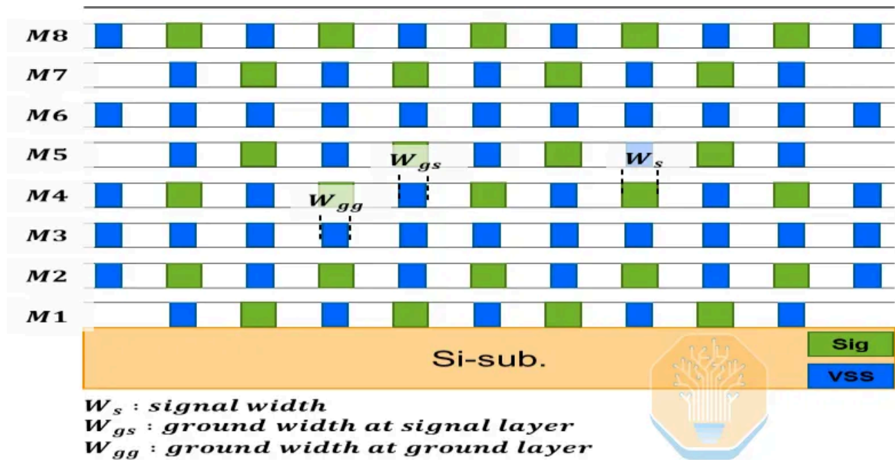
8-layer silicon interposer stack-up for HBM4E with two-signal / one-ground routing. Source: Samsung, “Advanced SI/PI Interposer Design Solution Enabling High-Performance HBM4e at up to 12Gbps,” ECTC 2026
