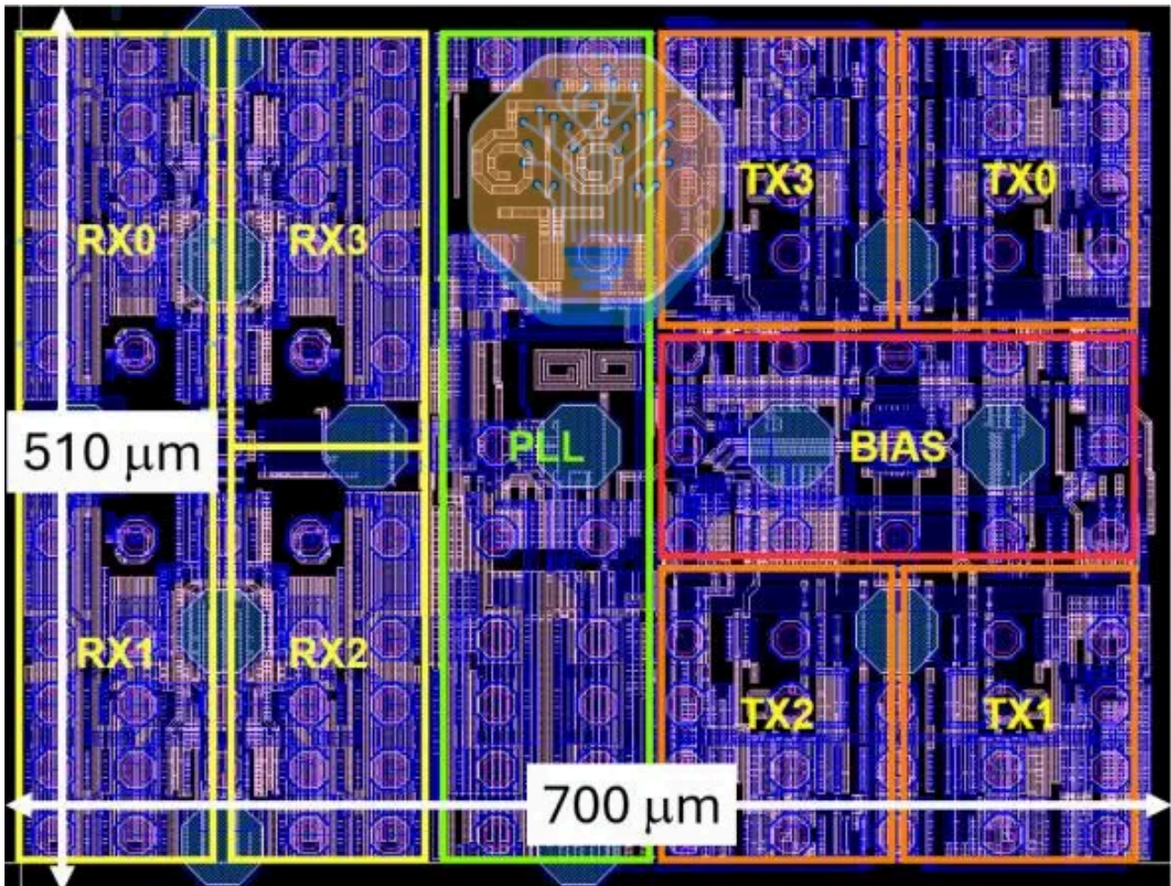
Photonic Fabric optical link test chip EIC with four TX-RX pairs. Source: Marvell, "Photonic Fabric™ Interconnect for a Scale-up Network Solution in Accelerated Computing," ECTC 2026
