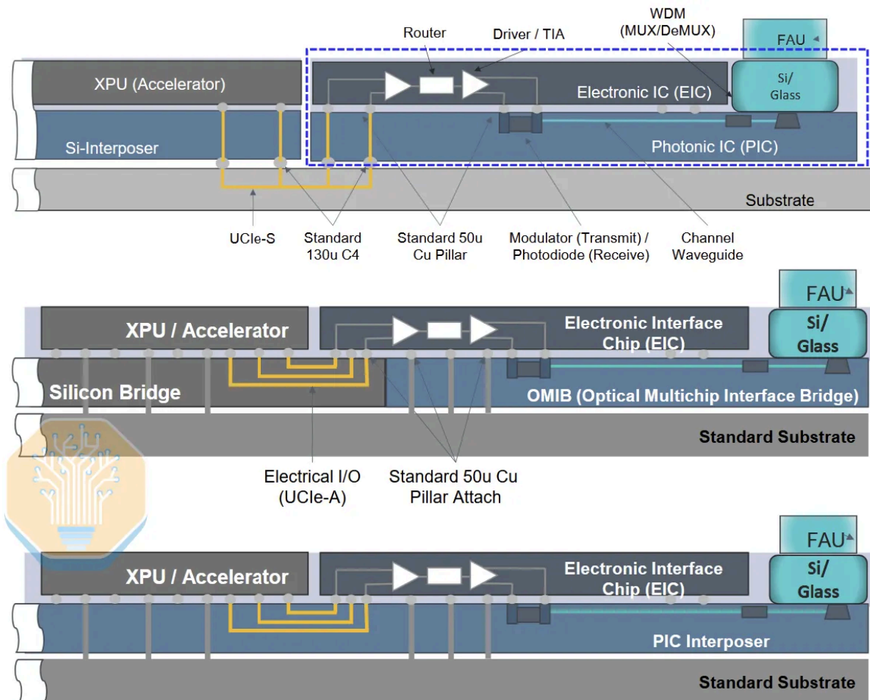
Package concepts with optical engine on substrate, OMIB and photonic interposer. Source: Marvell, "Photonic Fabric™ Interconnect for a Scale-up Network Solution in Accelerated Computing," ECTC 2026
