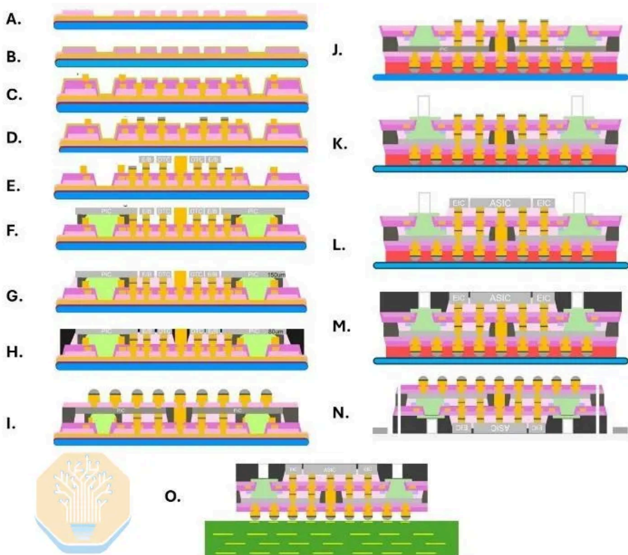
Process flow of 2.5D OMIB integration. Source: Marvell, "Optical Multi-Chip Interconnect Bridge (OMIB) Interposer Demonstration to Enable High-density Photonic Interconnects for High-Performance Computing Applications," ECTC 2026
