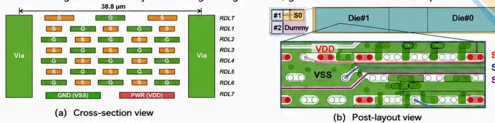
Fig. 3. CoWoS-R 8RDL physical design on RDLs. (a) Cross-section view; (b) post-layout view
