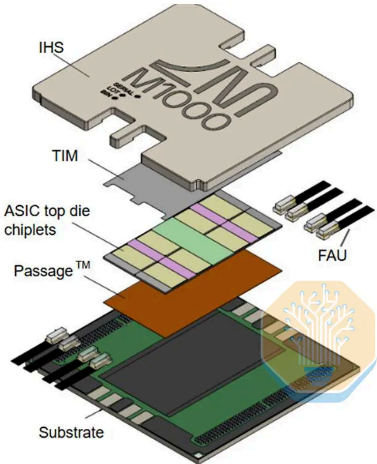
Passage M1000 schematic. Source: Lightmatter, “Advancing Interconnect Performance and Reliability with Innovations in 3D Photonic Integration Packaging and Fiber Coupling,” ECTC 2026
