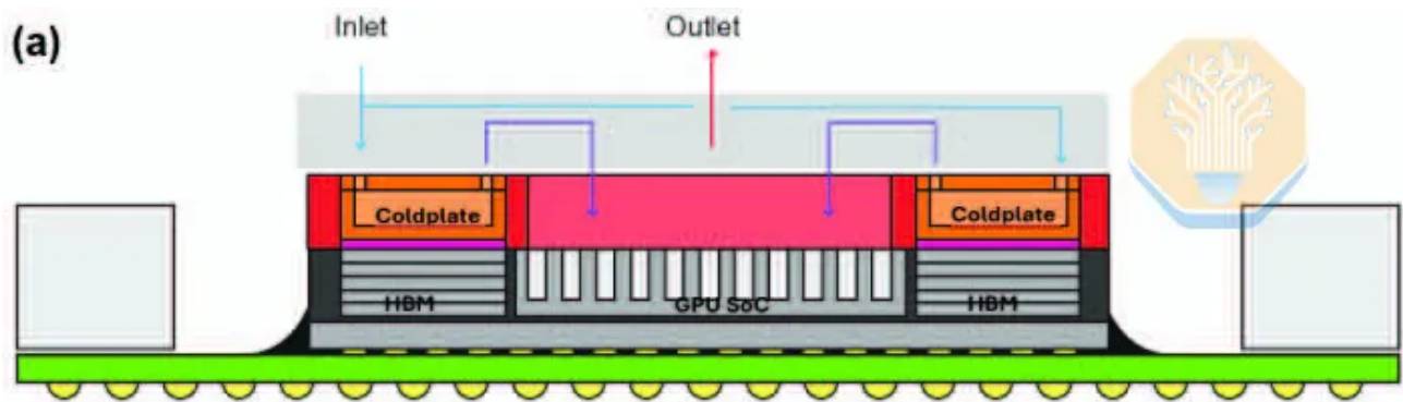
Microsoft's direct-to-silicon microfluidic cooling assembly for Nvidia GH200. Source: Microsoft, "Direct to Silicon Microfluidic Cooling for Datacenters," ECTC 2026
