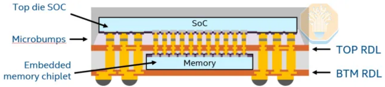
Schematic cross-section of FO-EB with embedded memory chiplet. Source: Intel and SPIL, “3D Integration of an SRAM chiplet in Fan-Out Embedded Bridge Platform Achieving Low Energy Read/Write,” ECTC 2026
