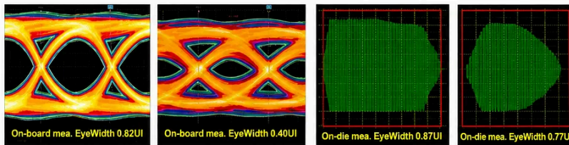
Fig. 7. UCle-A silicon measurement with 16 and 32 GT/s.
