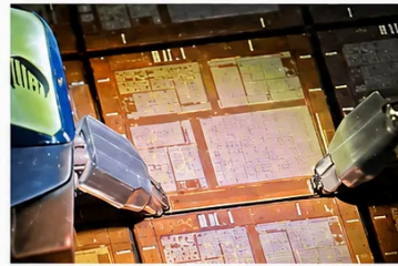
Fig. 6. UCle-A interconnect test keys design & correlation.
