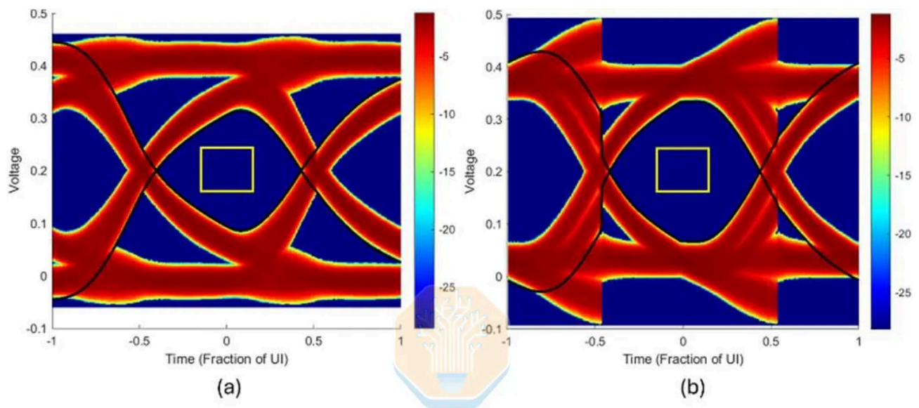
Signaling performance of HBM4E EMIB-T channel at 12 Gb/s without and with DFE. Source: Intel, "Enabling 12+Gb/s HBM4E with EMIB-T Advanced Packaging Technology," ECTC 2026
