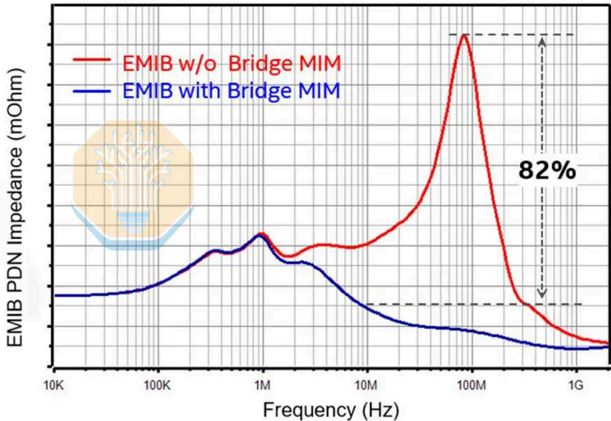
EMIB-T package PDN AC impedance for HBM4E with and without bridge MIM capacitors. Source: Intel, "Enabling 12+Gb/s HBM4E with EMIB-T Advanced Packaging Technology," ECTC 2026
