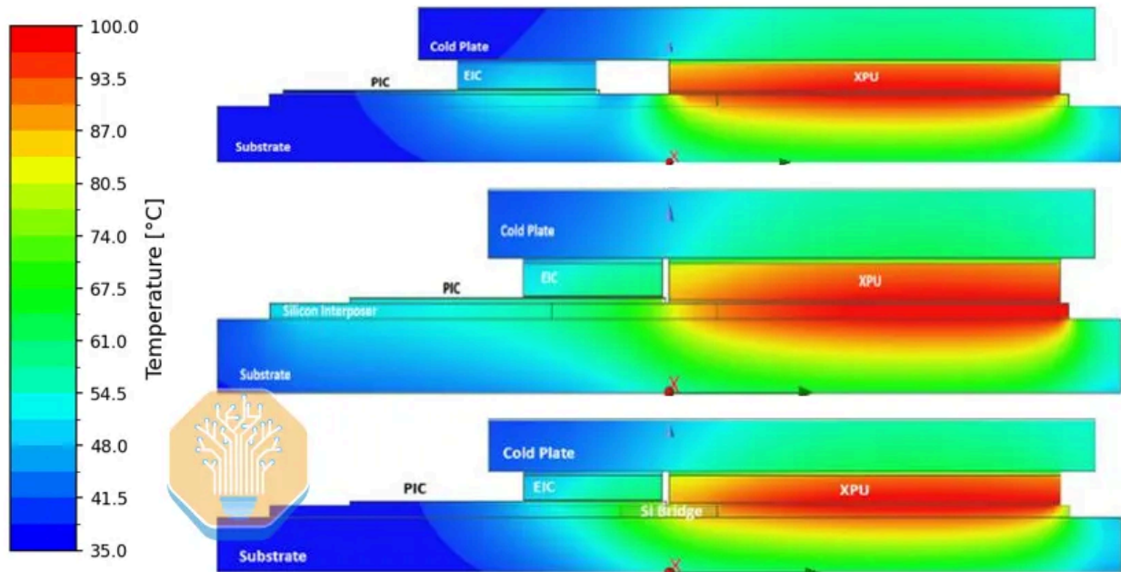
PIC steady-state temperature gradient under full XPU power on substrate, silicon interposer and silicon bridge. Source: Marvell, “Photonic Fabric™ Chiplets for Co-Packaged Optics in AI Data Centers,” ECTC 2026
