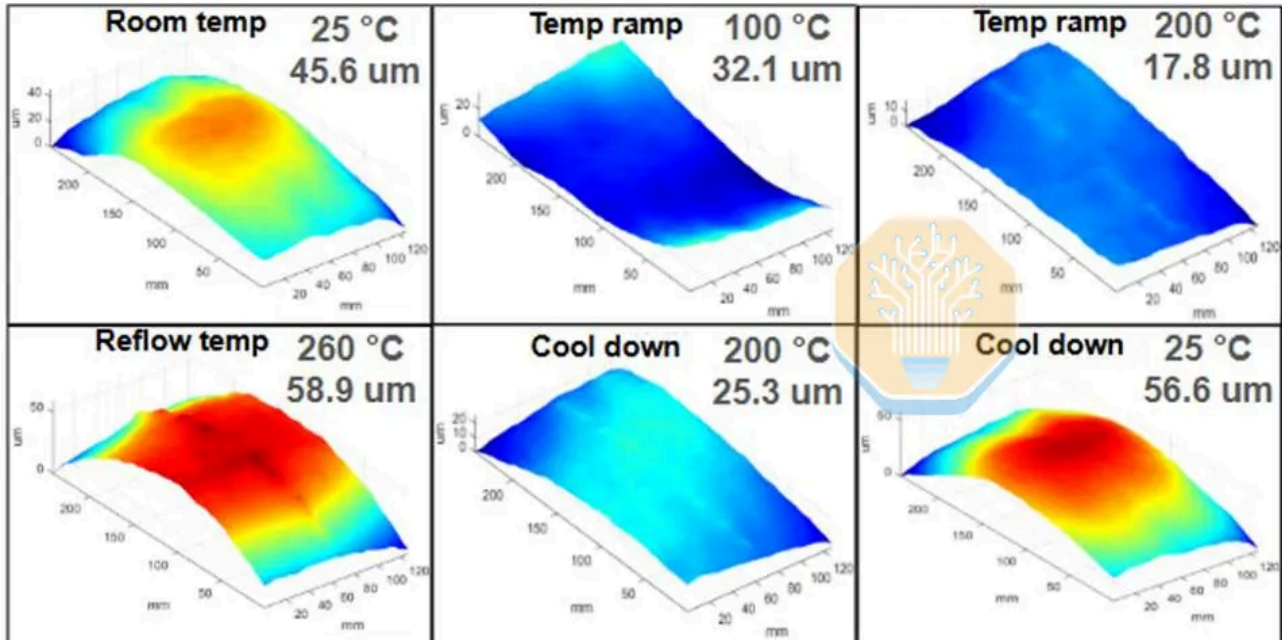
Passage M1000 package warpage during temperature ramp-up and cool-down. Source: Lightmatter, “Advancing Interconnect Performance and Reliability with Innovations in 3D Photonic Integration Packaging and Fiber Coupling,” ECTC 2026
